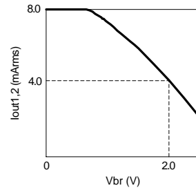
Dimming characteristic (Reference)
